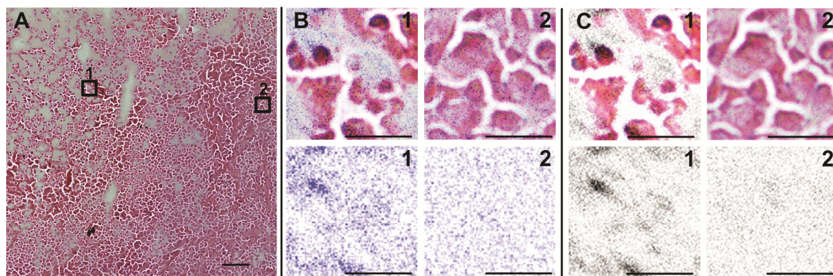
Figure 5: (A) Optical image of a small part of MDA-MB-231 tumor, stained with H&E after concluding a MetA-SIMS experiment with (1) necrotic region and (2) viable tumor areas selected. (B) Na^+ and (C) K^+ distribution from MetA-SIMS data and overlay with microscopic image in regions (1) and (2) are shown the upper part; the individual ion distributions on areas (1) and (2) are shown at the bottom. Due to previous gold coating of the tissue, the hematoxylin staining was less efficient, therefore the visibility of cell nuclei is less pronounced. Scale bar: (A) 100 \mu m ; (B) and (C) 25 \mu m .
